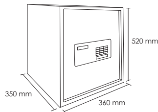
iSB-04 360x520x350mm
